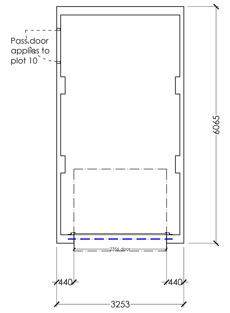
Single Garage PLAN
