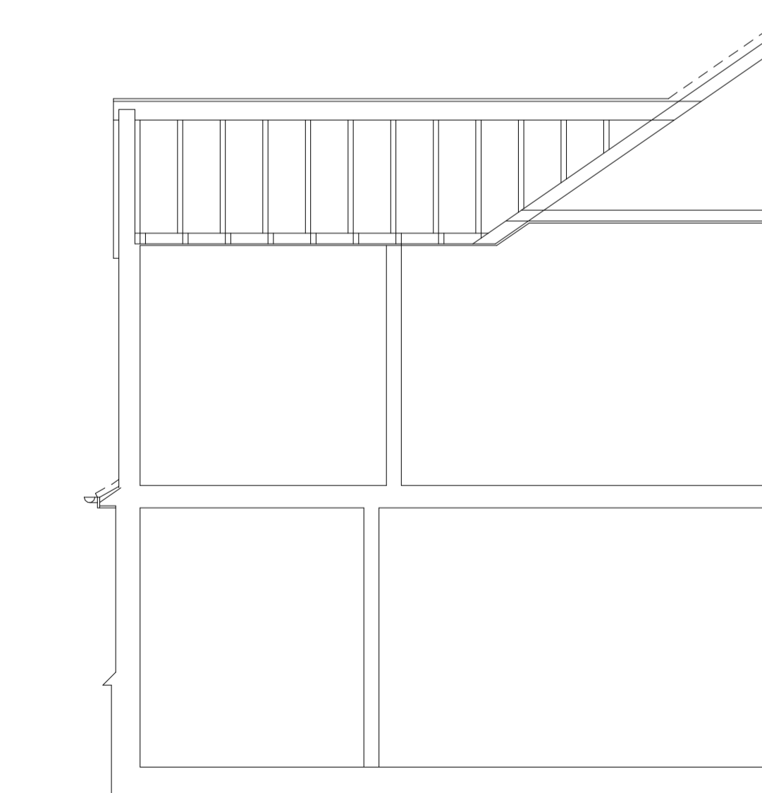
TYPICAL SECTION
