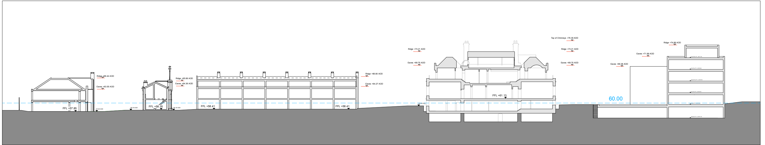
Section through site showing site levels and building heights
