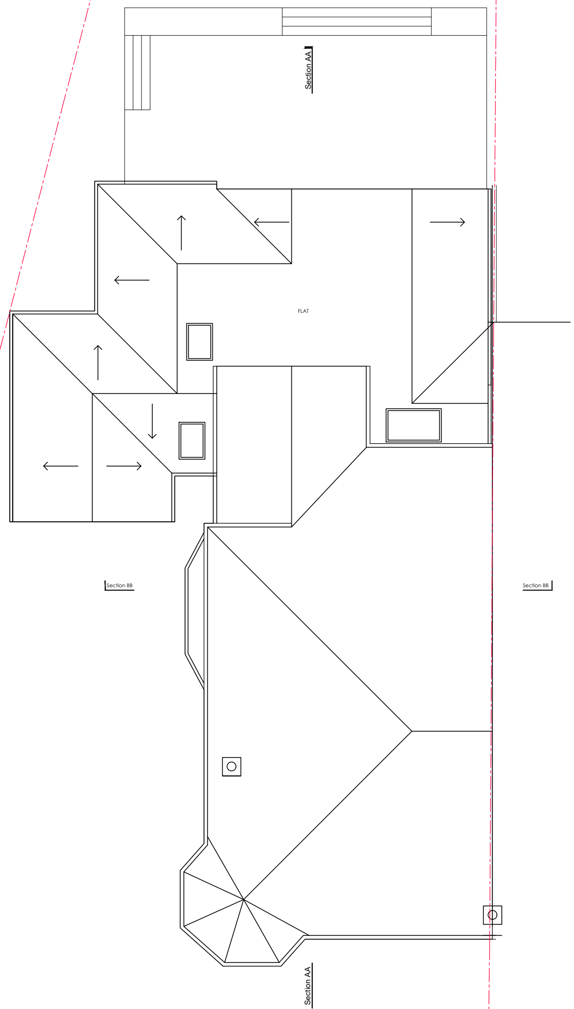
Roof Plan as Proposed @ 1:100
