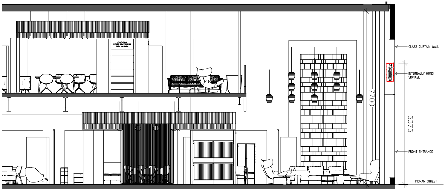
PART SECTION THROUGH SHOPFRONT FRONT ELEVATION TO INGRAM STREET
