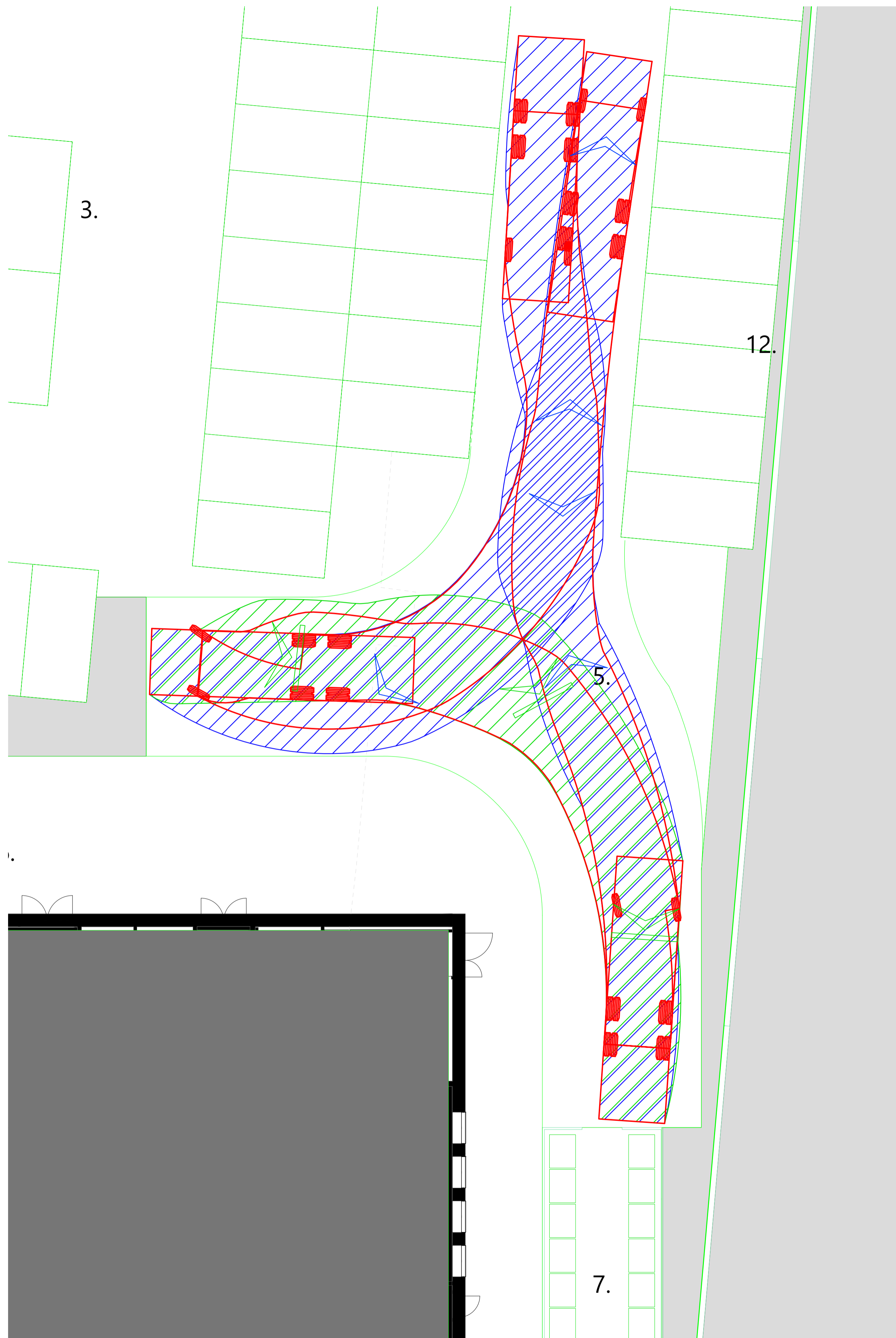
02 | Vulture 2225 (with Mercedes Econic 2628LL 6x4 chassis) SCALE: 1/100
