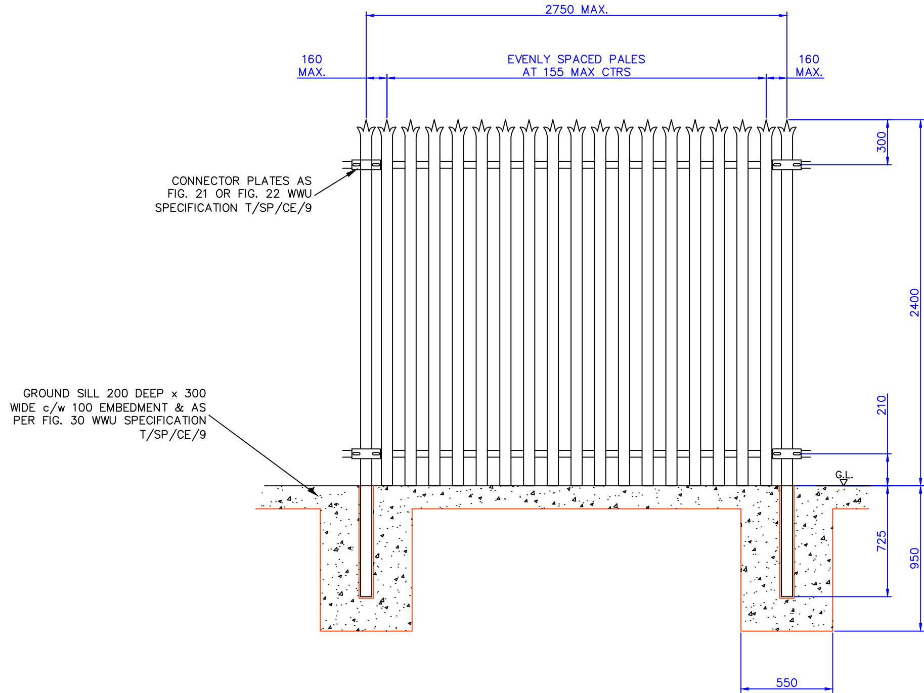
1 2.4m HIGH FENCING PANEL 1:25 GENERALLY IN ACCORDANCE WITH WWU SPECIFICATION T/SP/CE/9 FIG. 28 - FENCE REF. P1 ALL DIMENSION IN MM UNLESS OTHERWISE STATED
