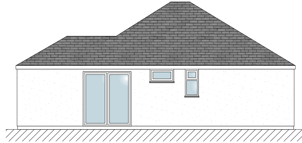
North East Elevation SCALE 1:100
