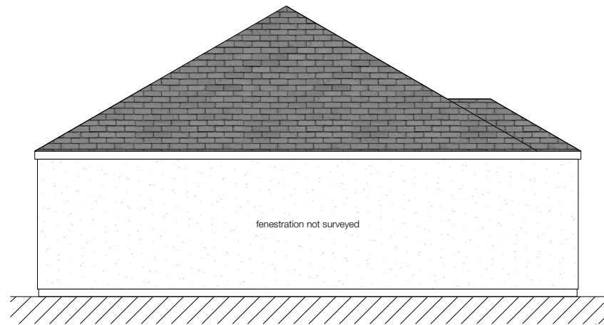
North West Elevation SCALE 1:100
