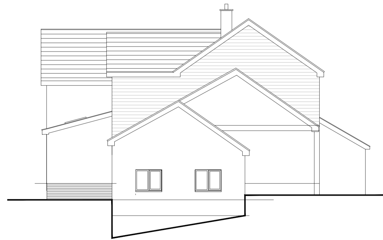
Side Elevation 1:100
