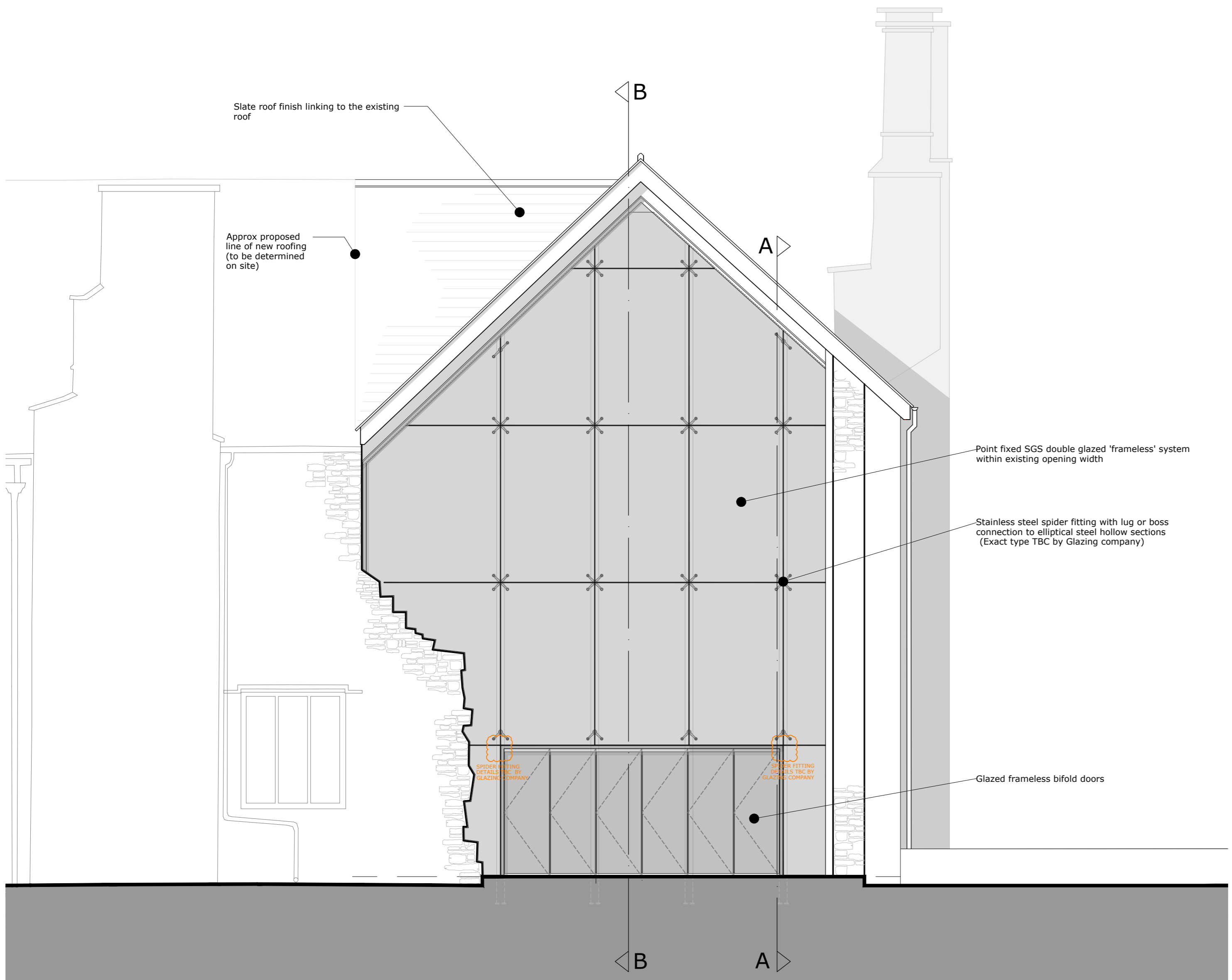
PROPOSED PART WEST ELEVATION
