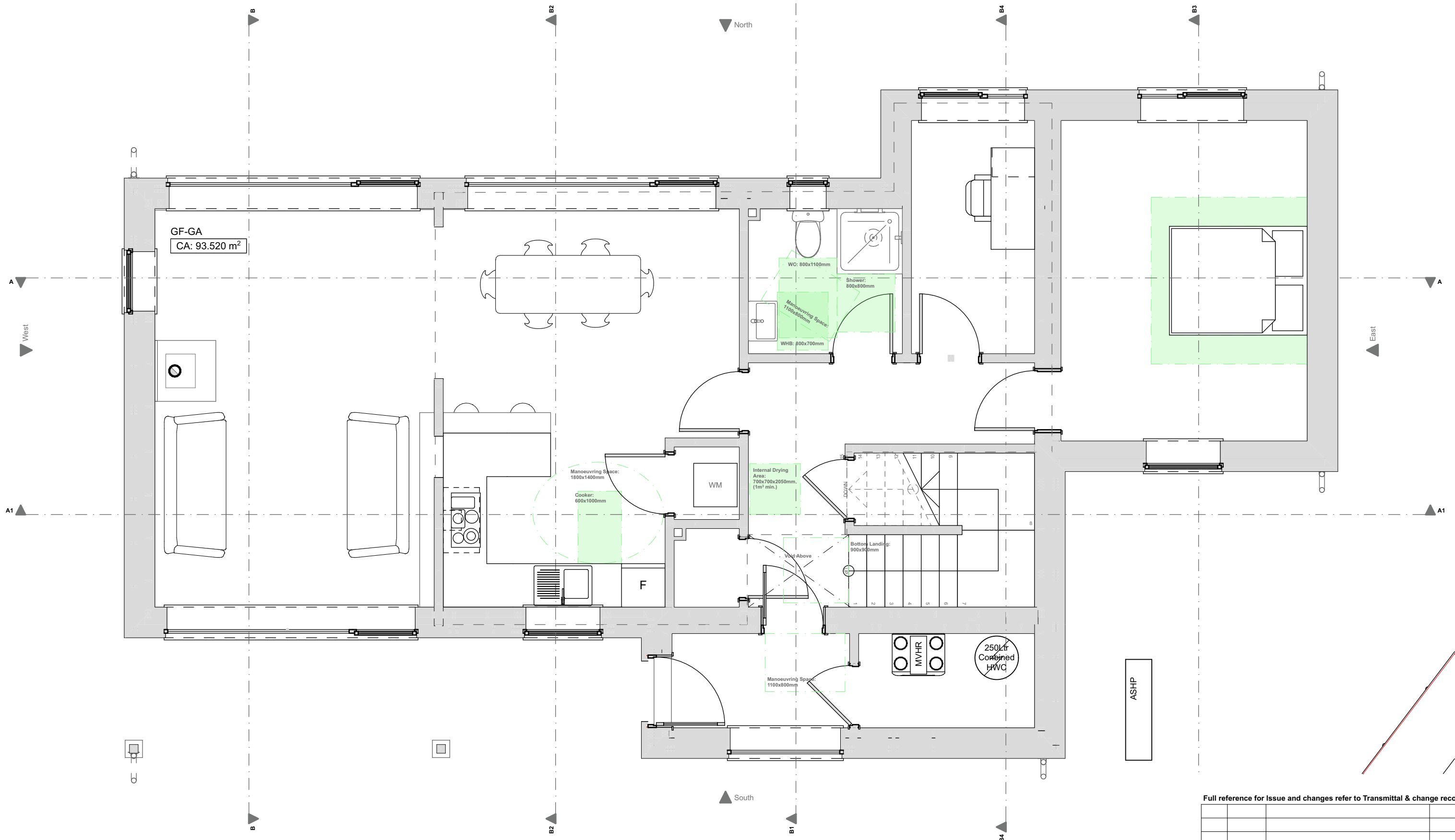
1 GF-Ground Floor 1:50
