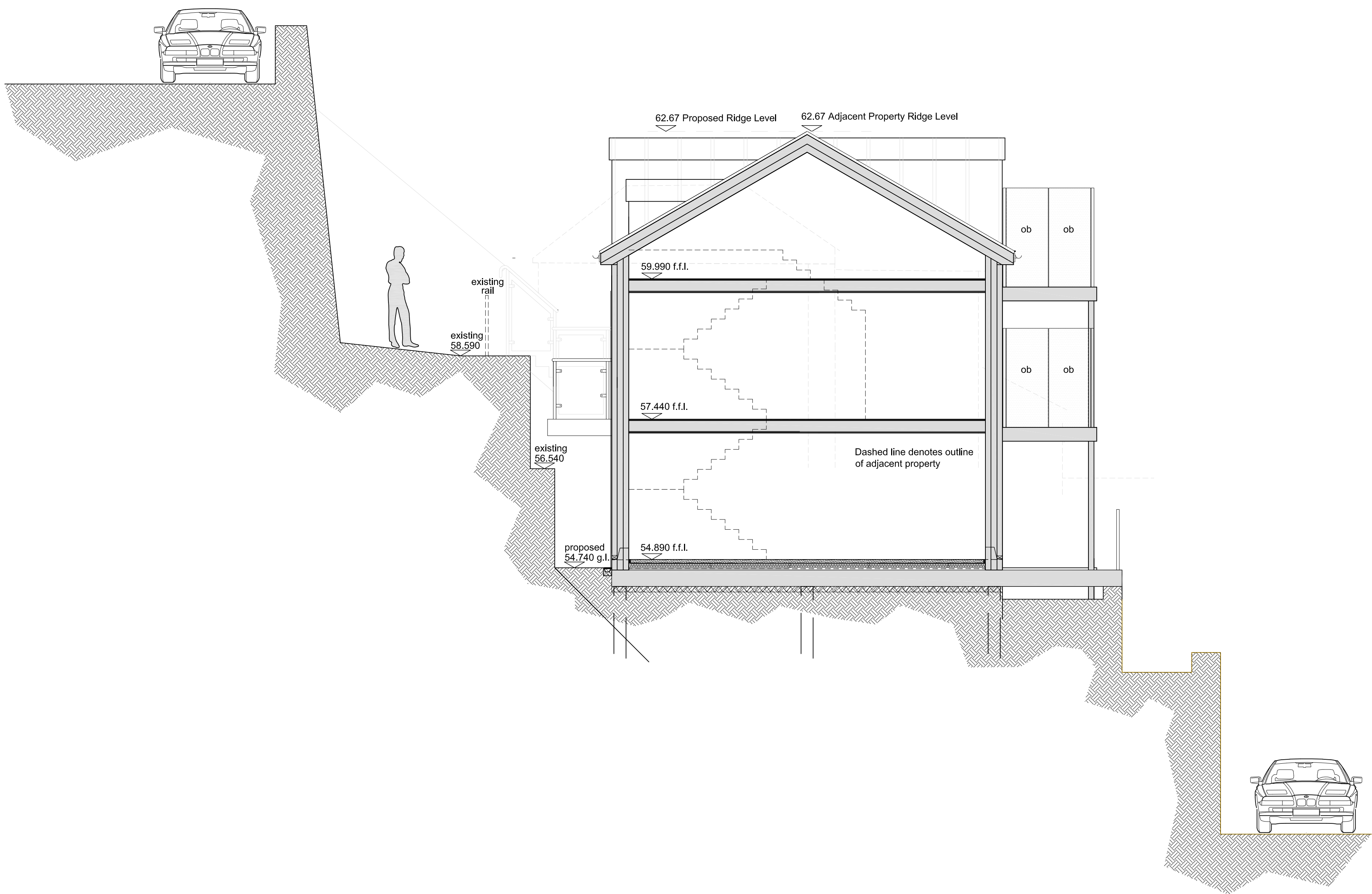
Proposed Side (North) Section 1:50
