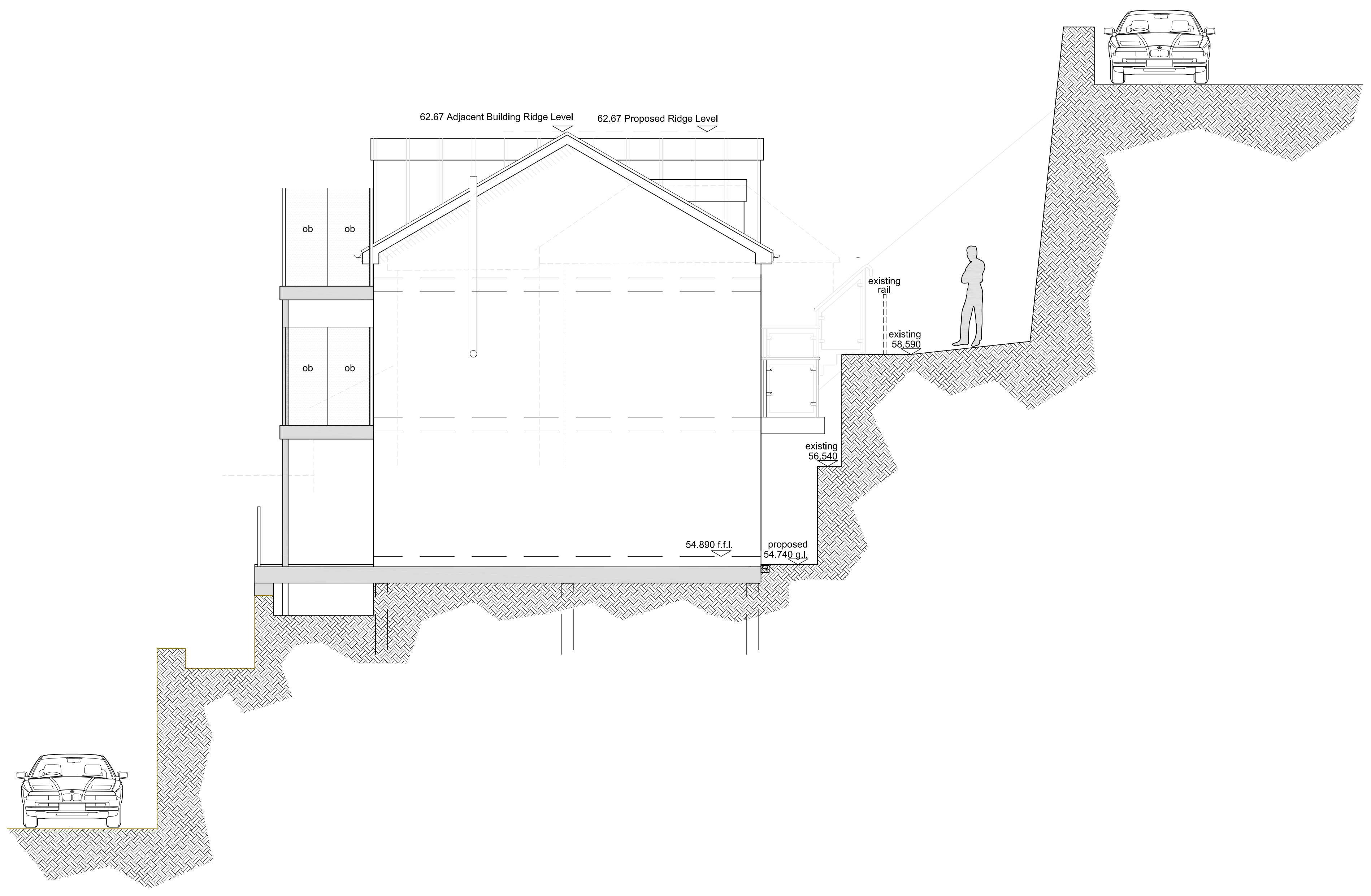
Proposed Side (South) Elevation 1:50
