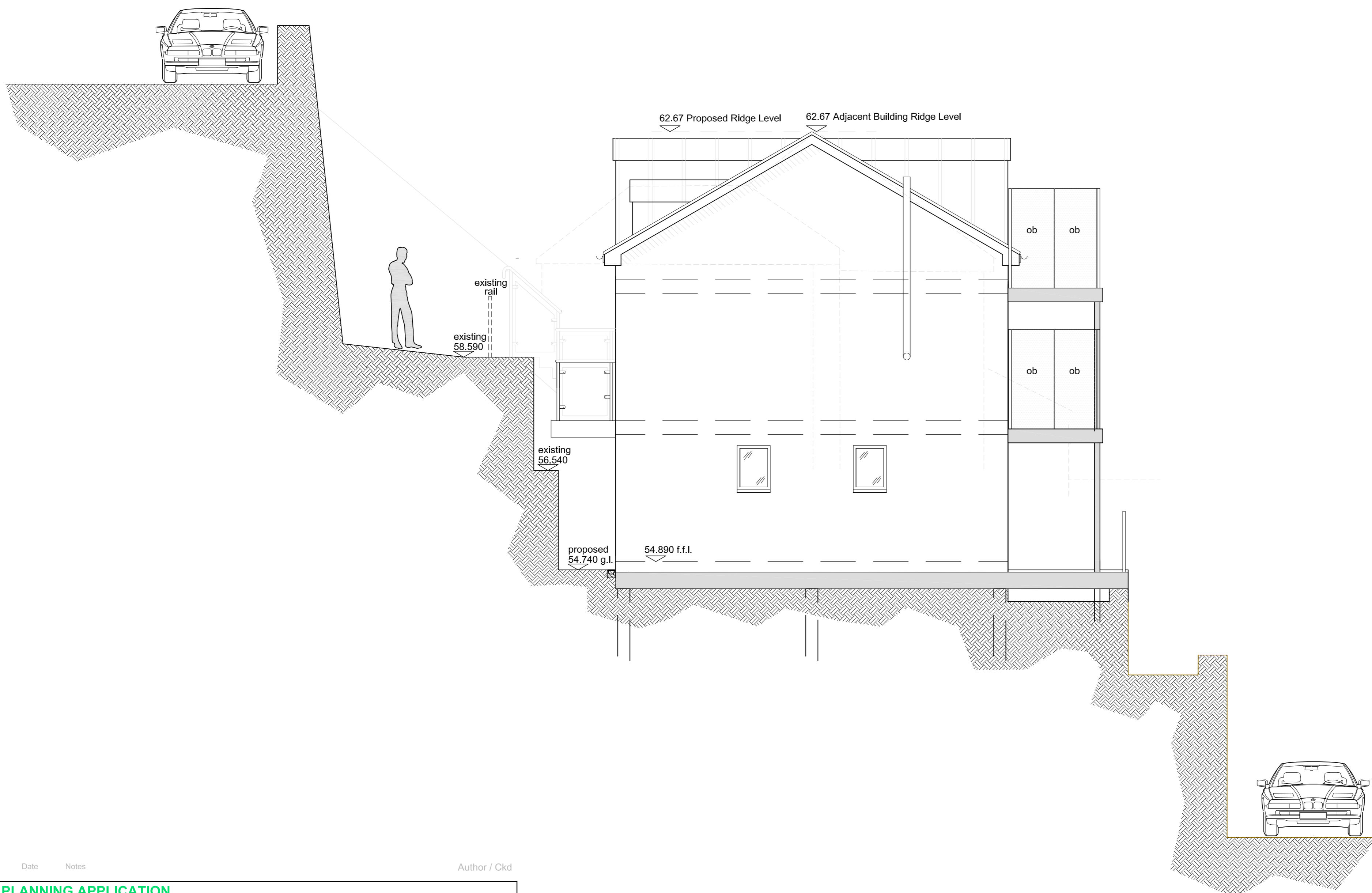
Proposed Side (North) Elevation 1:50
