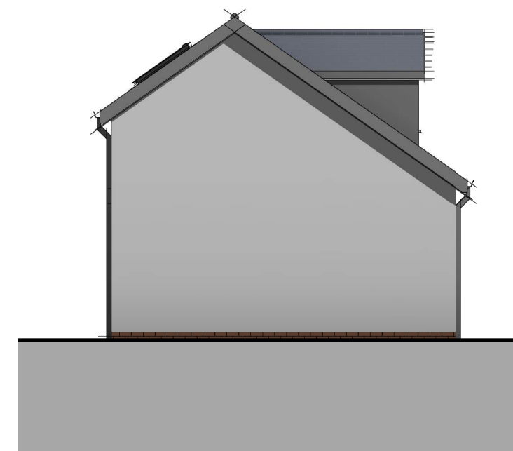
2 Side Elevation 1 (North-East) 1 : 100
