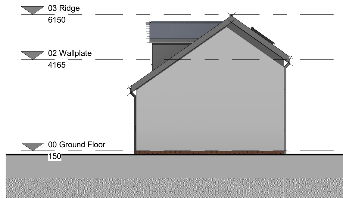
3 Side Elevation 2 (South-West) 1 : 100
