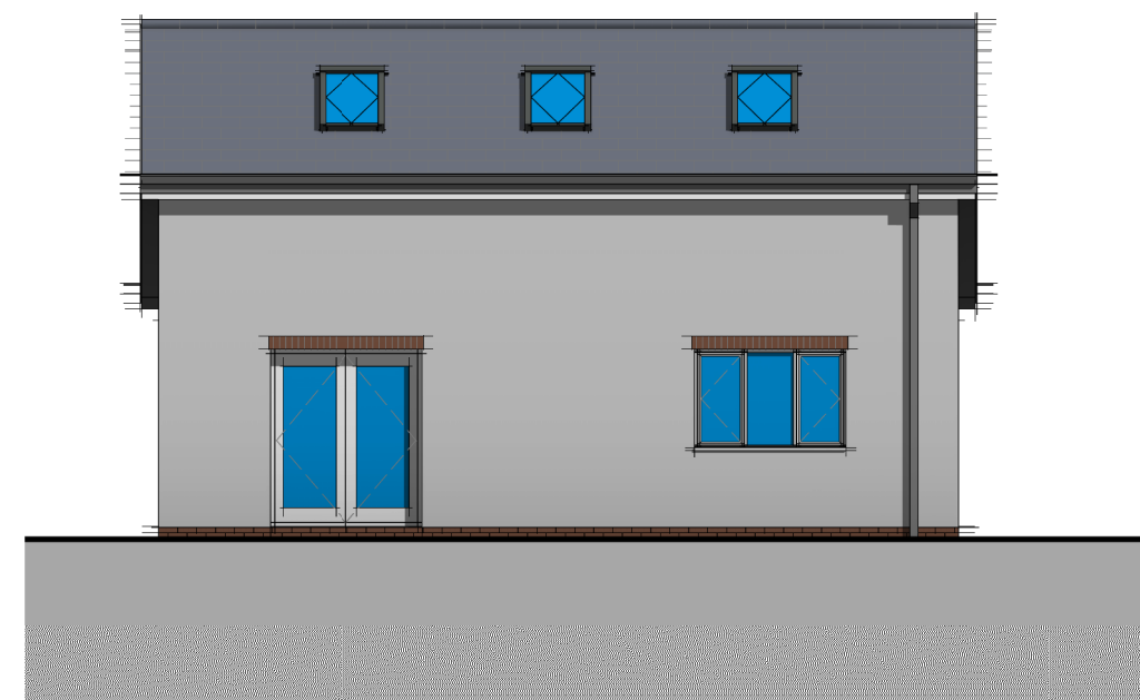
4 Rear Elevation (South-East) 1 : 100
