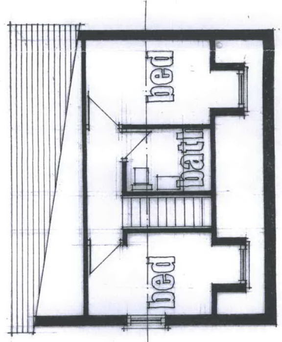
F-F plan
