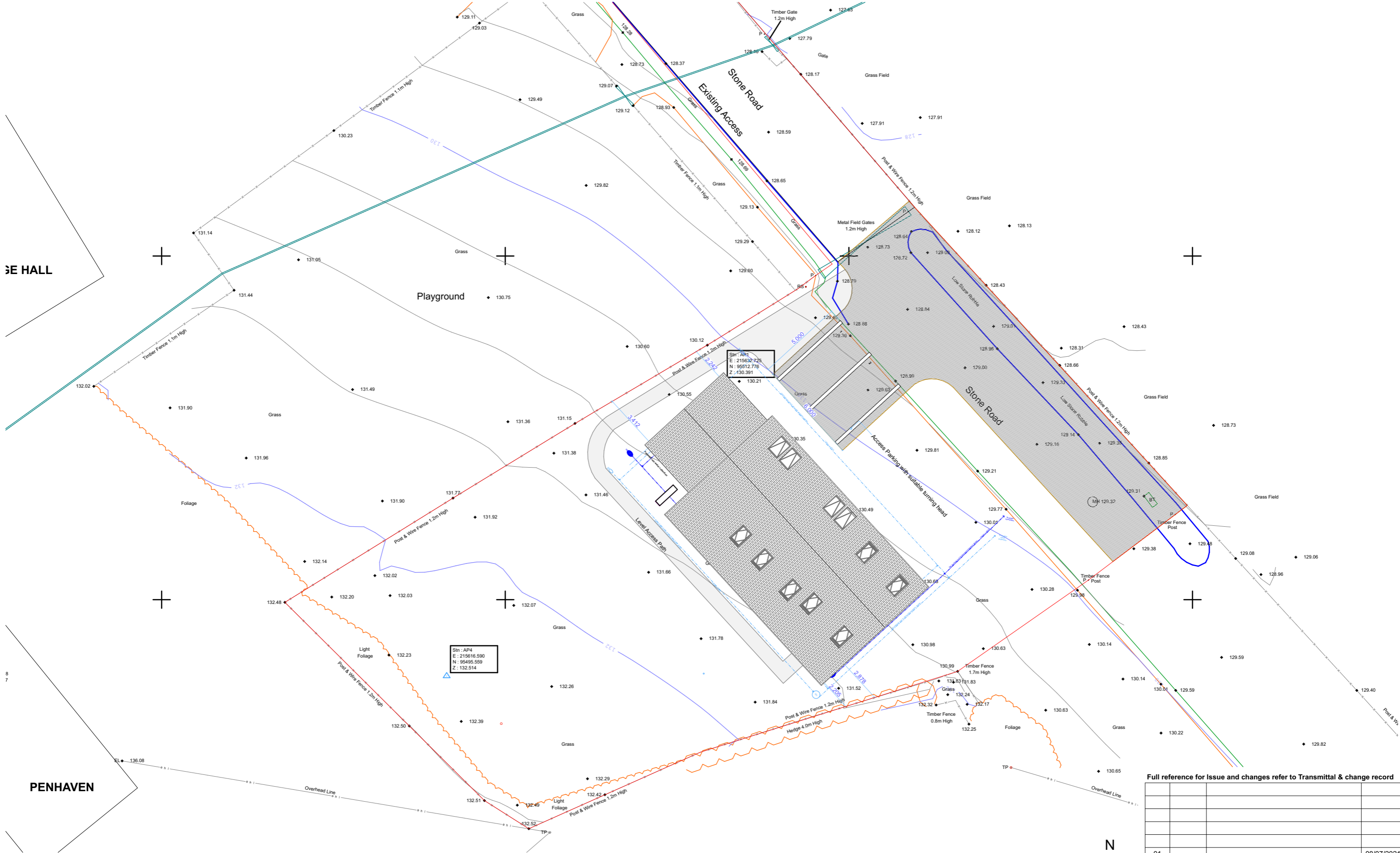
1 Site Plan Proposed 1:200
