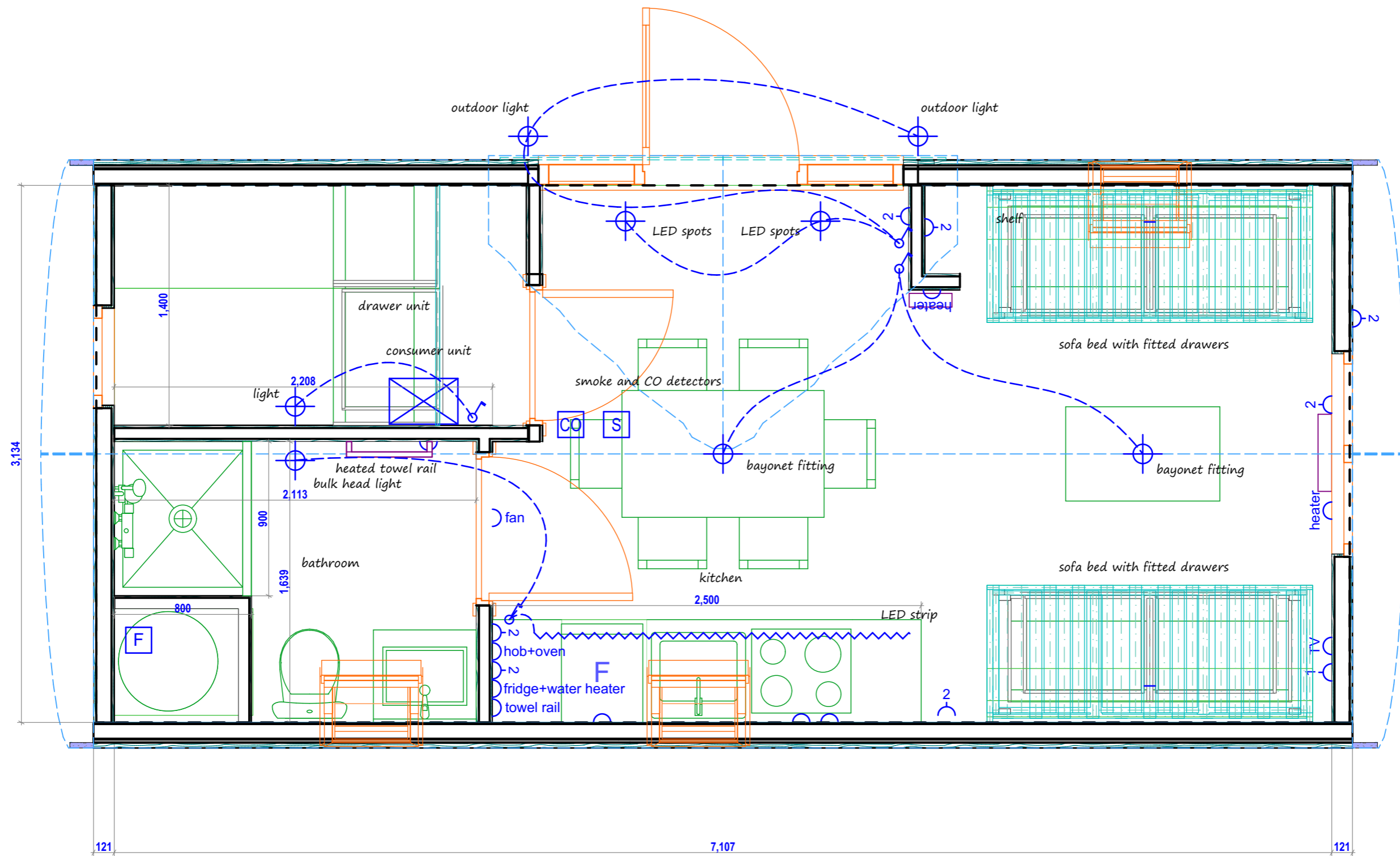
1 - cabin layout 1:25
