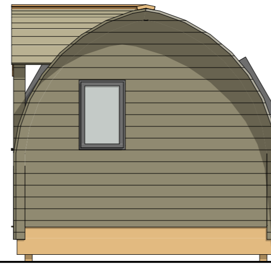
2 gable right elevation 1:50
