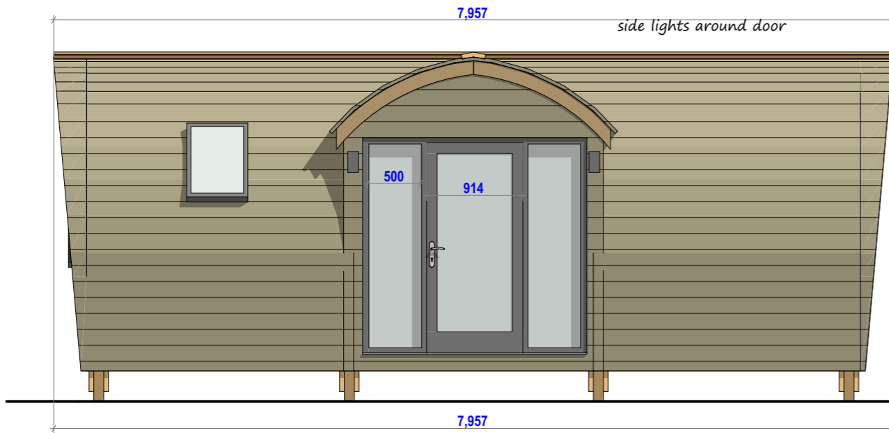
3 front elevation 1:50
