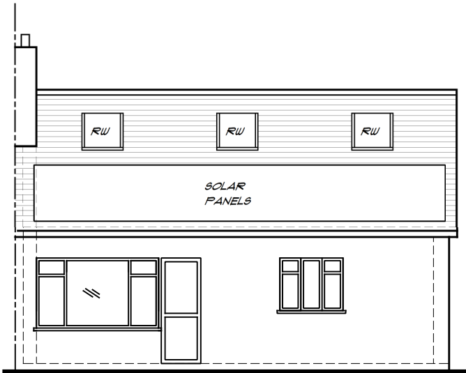
PRE-EXISTING REAR ELEVATION SCALE 1 : 100 (A3)
