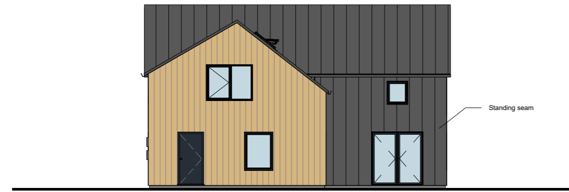
West Elevation 1 : 150
