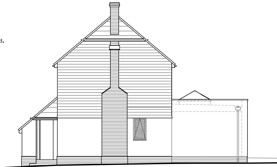
4 WEST SIDE ELEVATION
