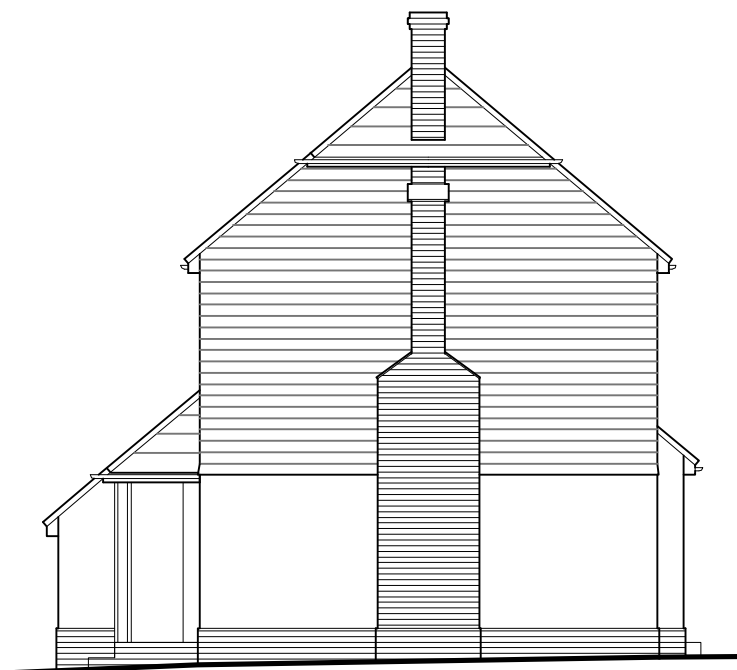
4 WEST SIDE ELEVATION
