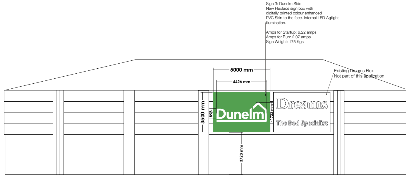
Side Elevation Drawing
