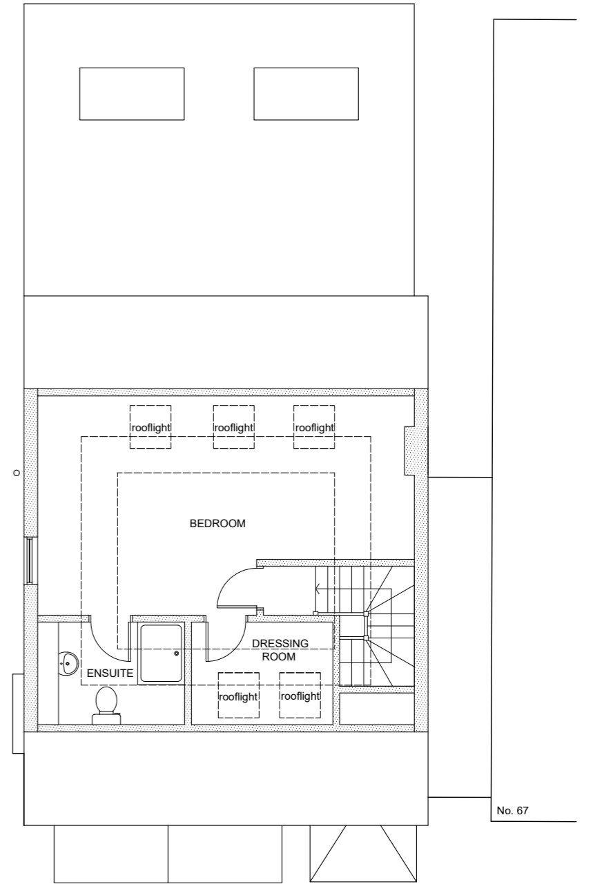
EXISTING LOFT PLAN 1:100
