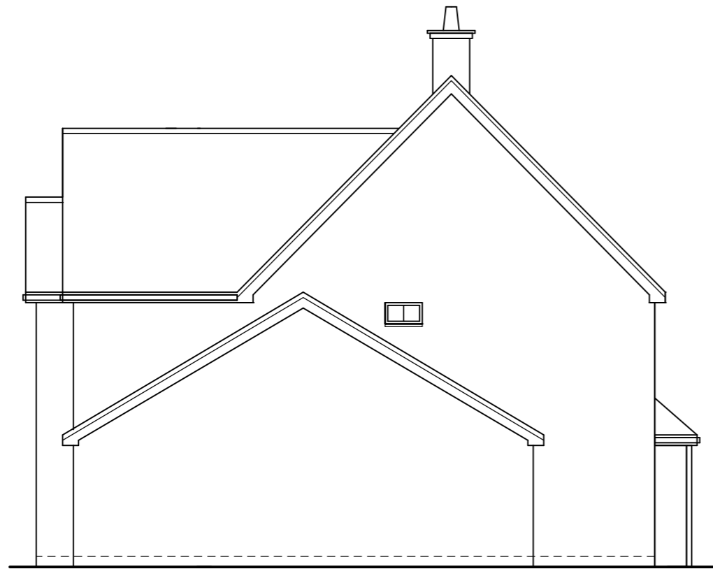
left side (southwest) elevation
