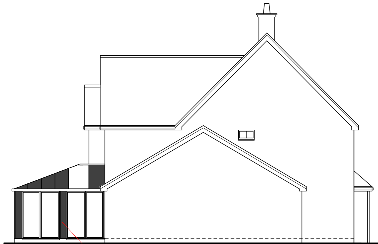
left side (southwest) elevation
