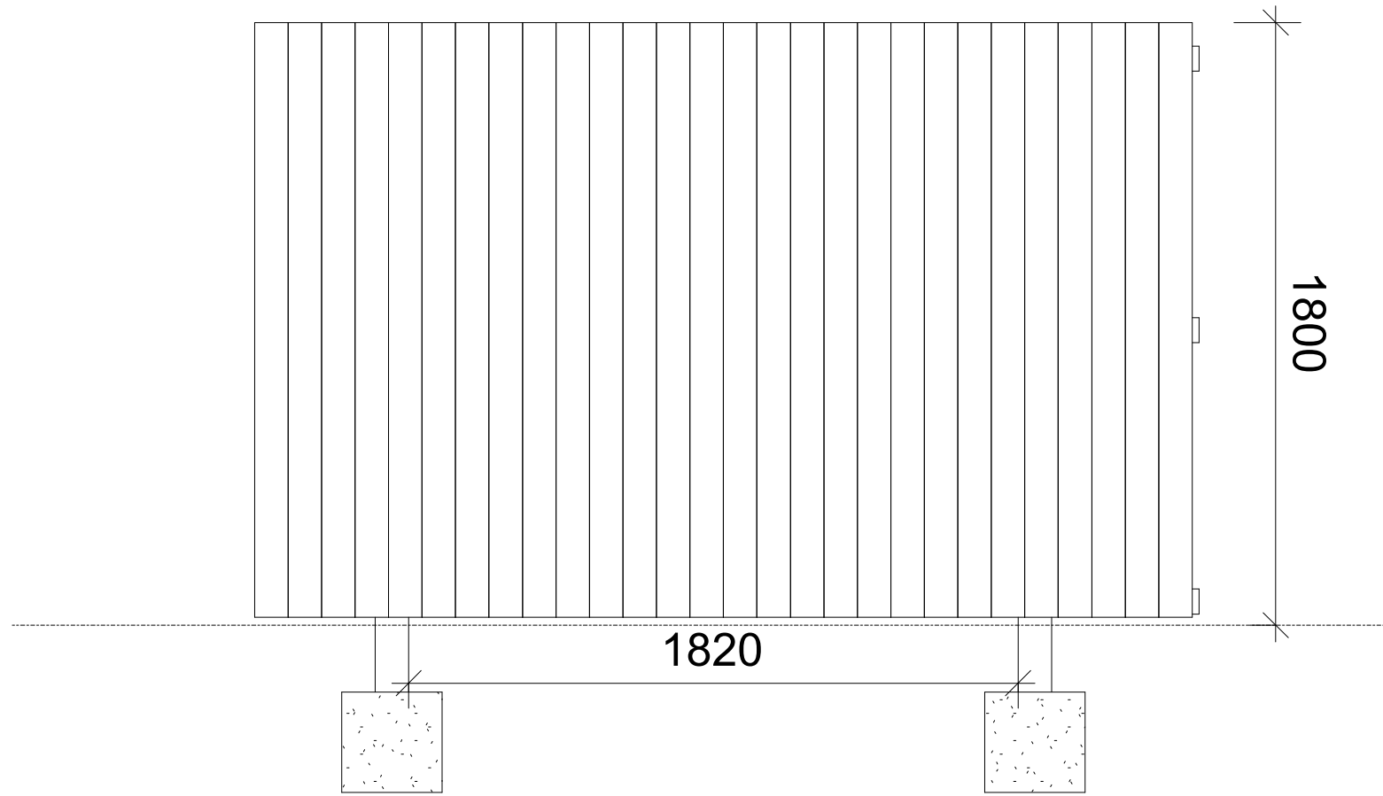
1.8m Timber Panel Fence Elevation 1 : 20
