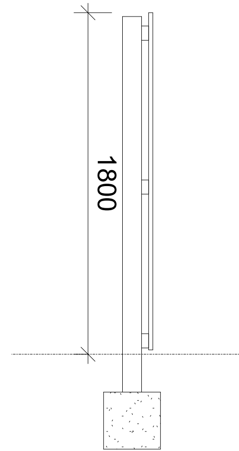
1.8m Timber Panel Fence Section 1 : 20
