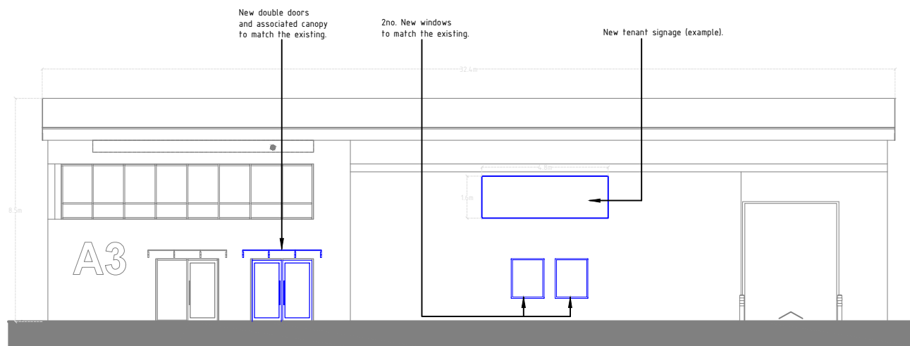
West Elevation.
