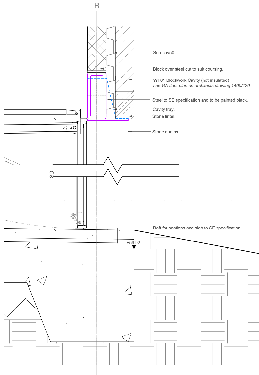
01 - D0.01/01 Head and Cill Detail
