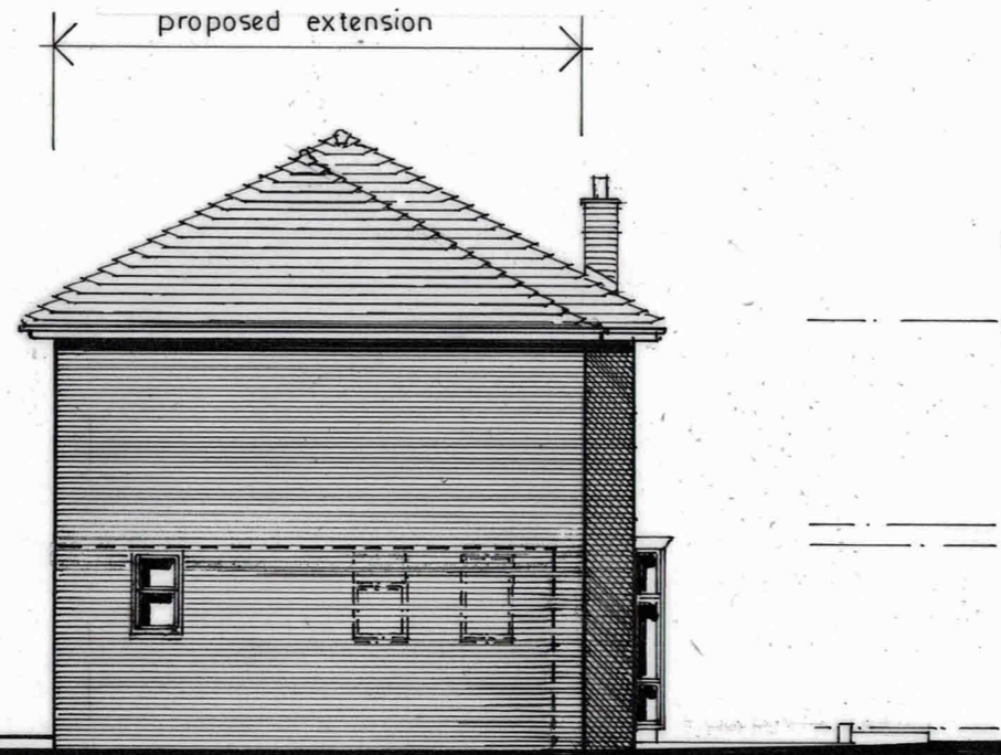
SIDE ELEVATION east 1:100
