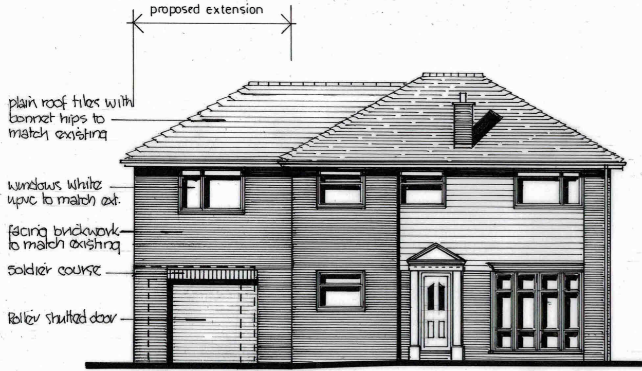
FRONT ELEVATION north 1:100
