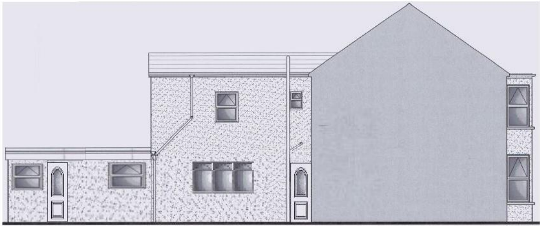
Side Elavation
