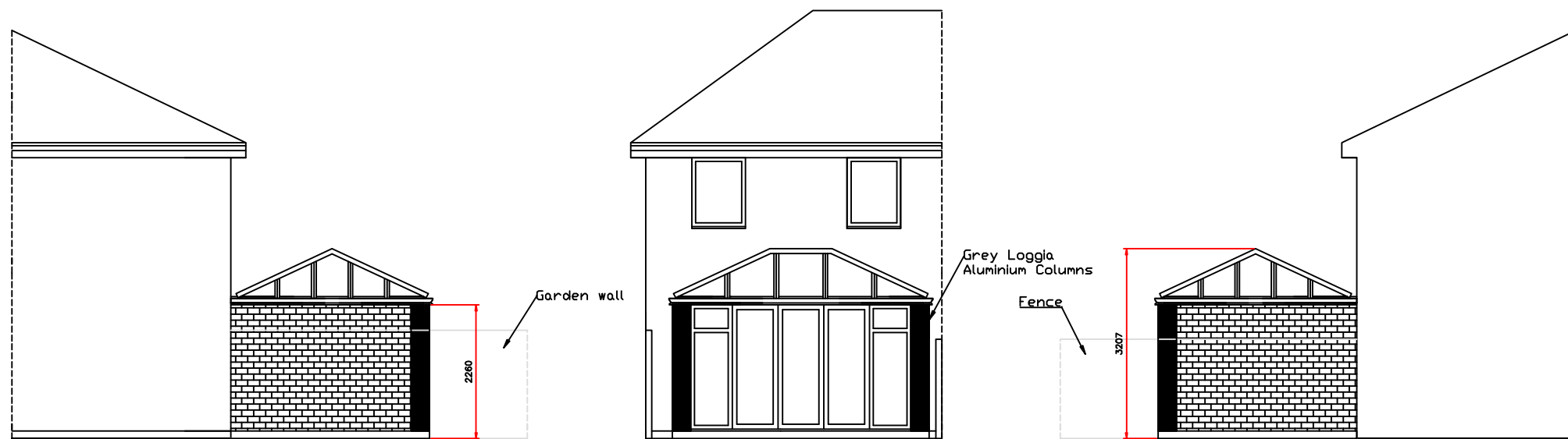
PROPOSED REAR LEFT HAND ELEVATION
