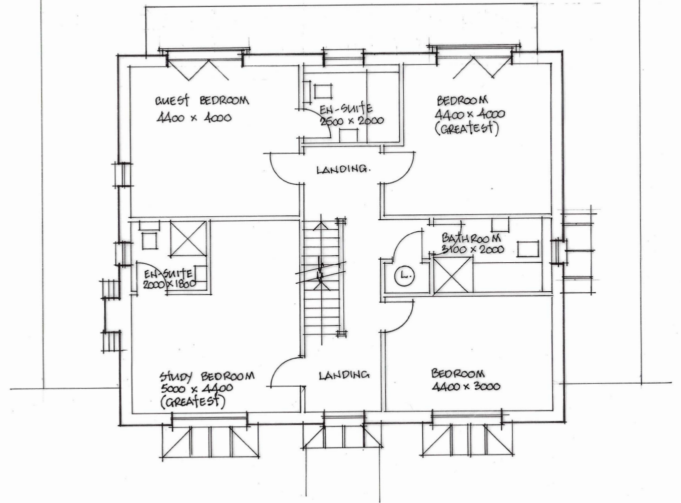
PLAN AT FIRST FLOOR LEVEL.
