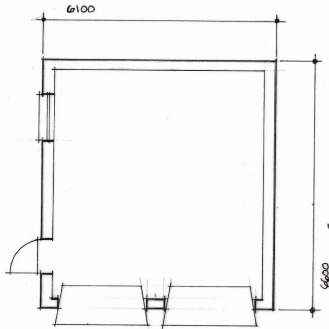
PLAN OF DOUBLE GARAGE.
