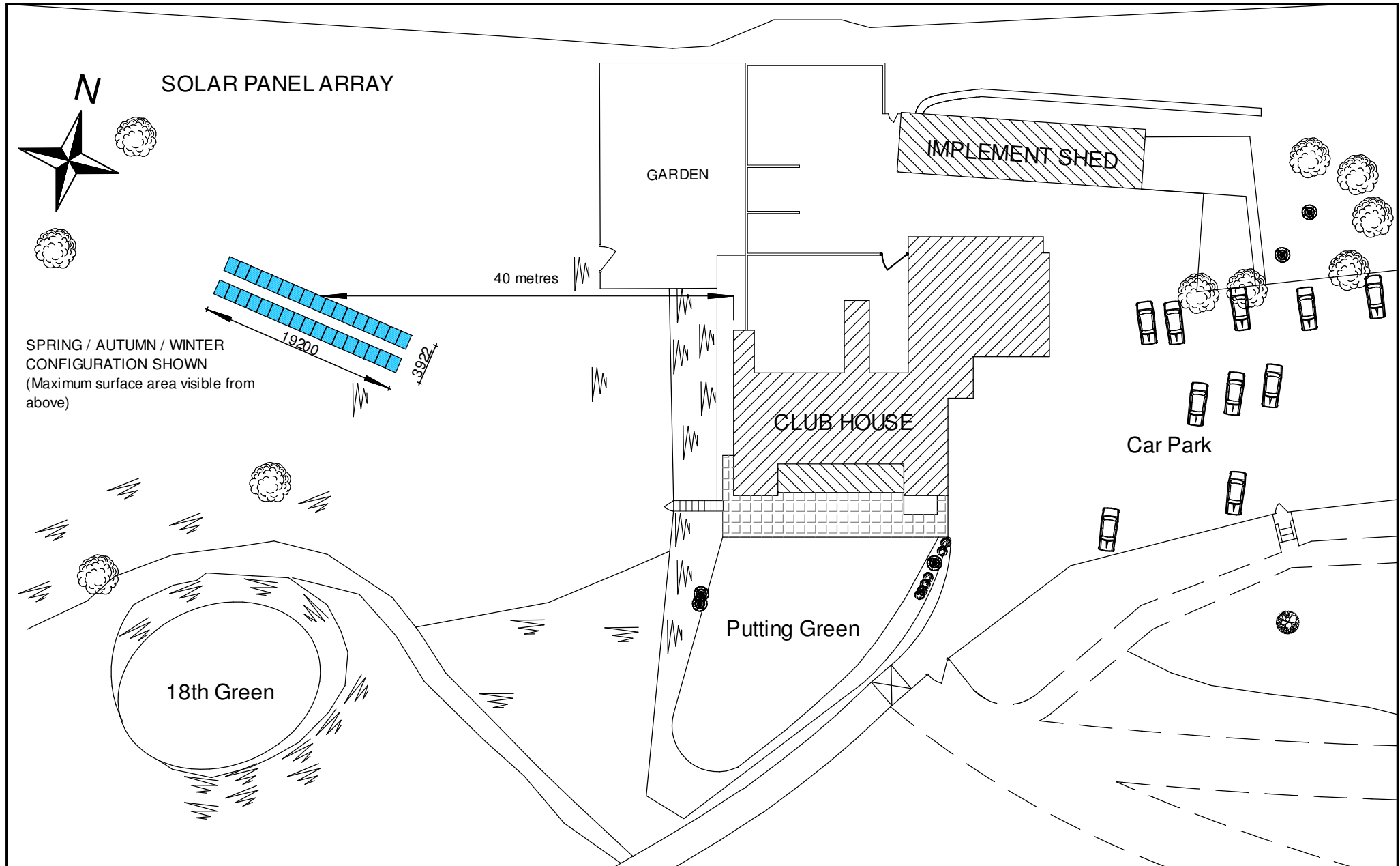
PROPOSED SOLAR PANEL ARRAY AT WELSHPOOL GOLF CLUB - SOLAR PANEL LOCATION PLAN
