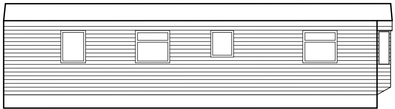
North Elevation 1:100
