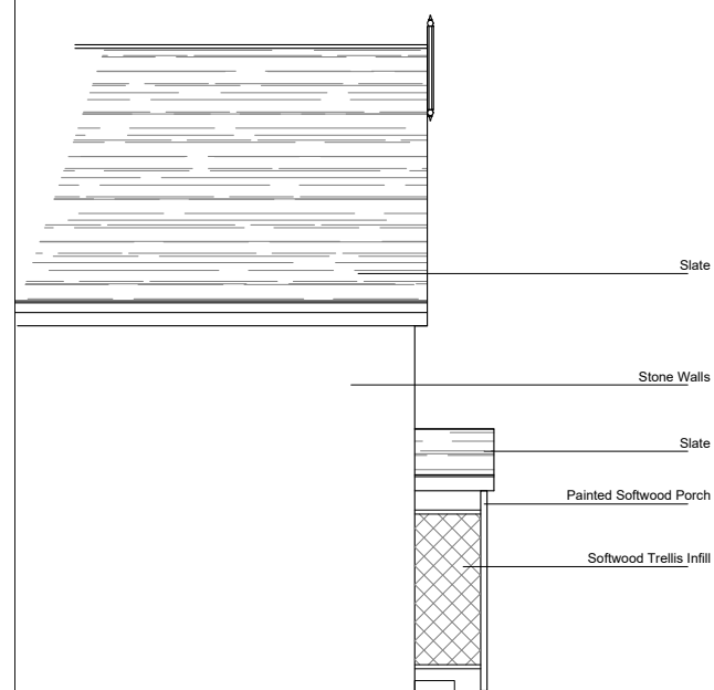
Existing Front Elevation. North West - (PART)
