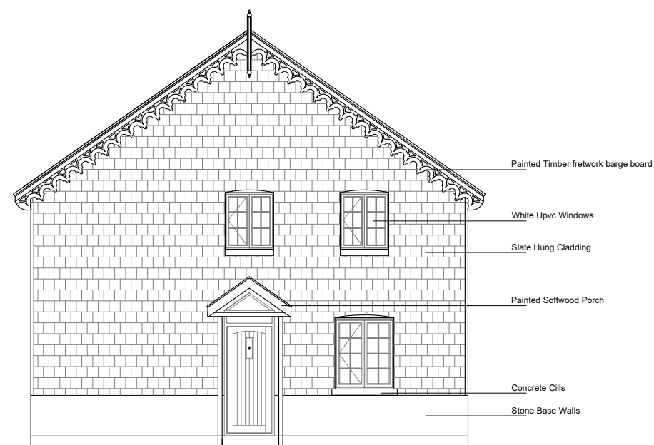
Existing Side Elevation. South West - (PART)
