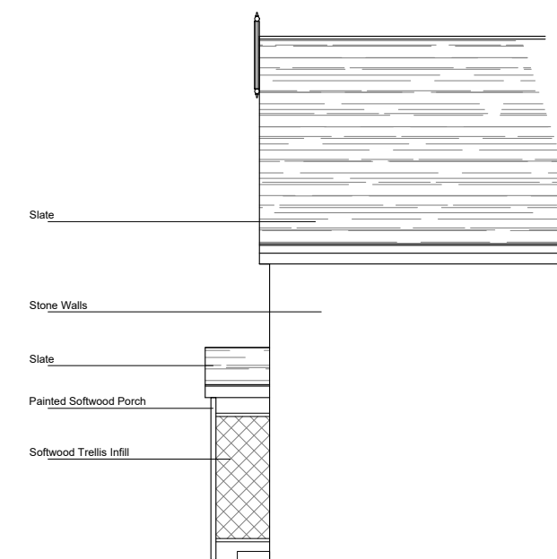
Existing Rear Elevation. South East - (PART)
