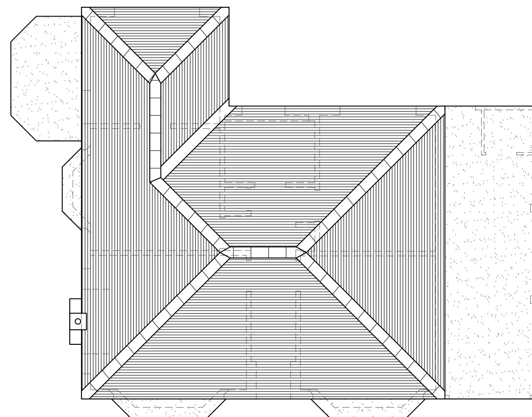
Roof Plan 1:100
