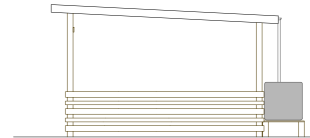
end elevation (North)
