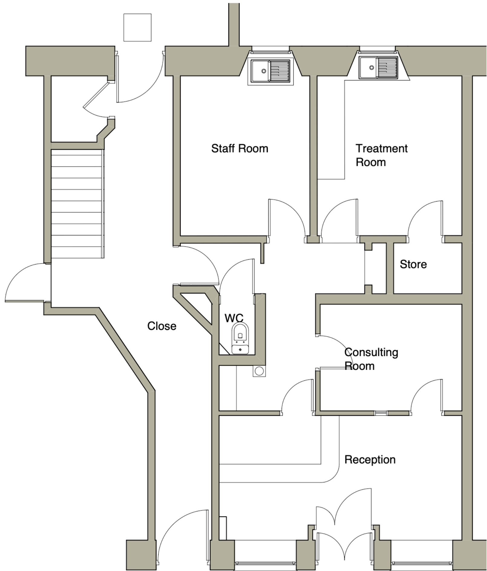
001 Existing Ground Floor Plan 1:50
