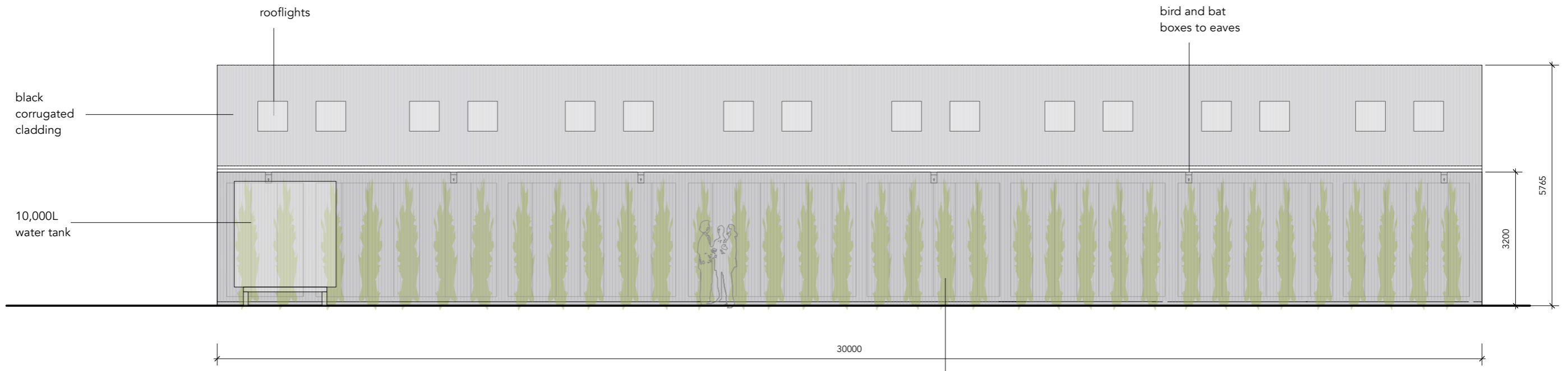
1 proposed north elevation
