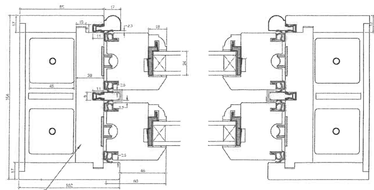
HORIZONTAL DETAIL
