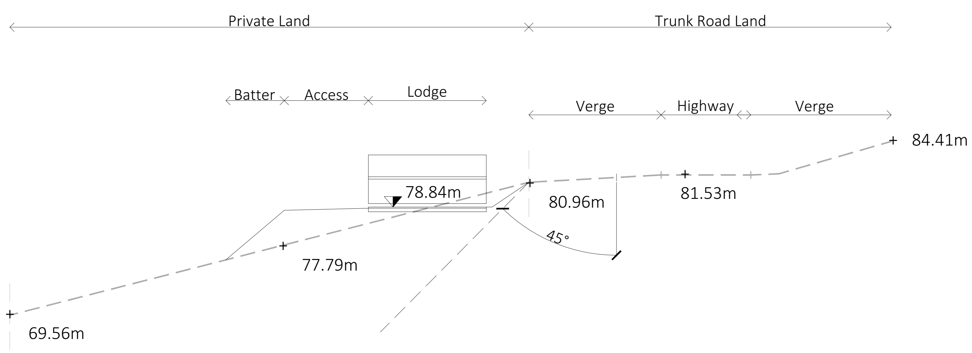
Section AA Lodge #1
