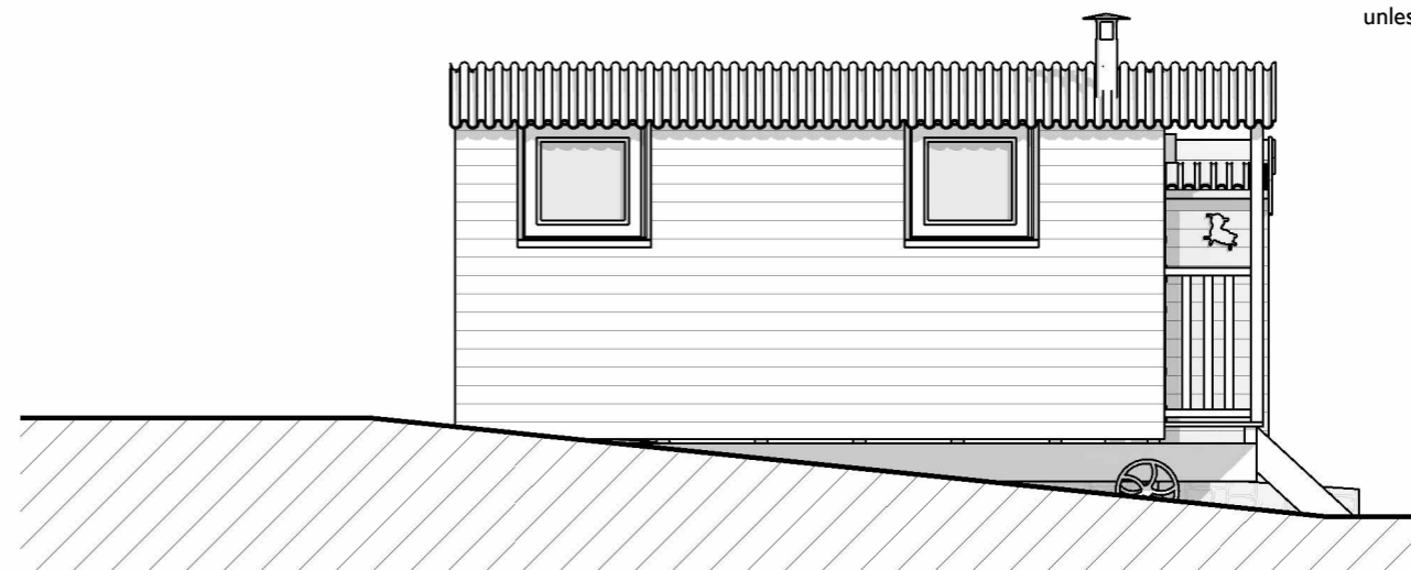
Side Elevation
