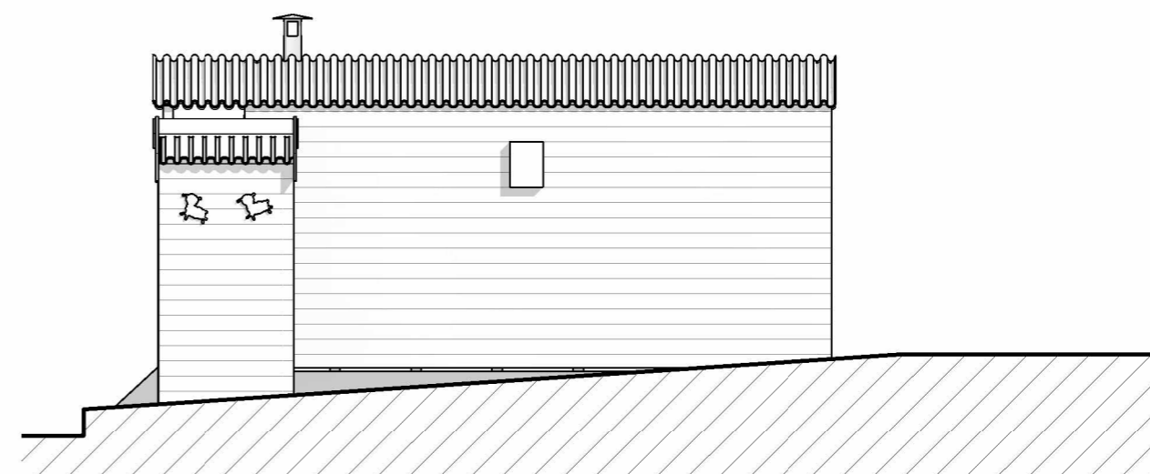
Side 2 Elevation
