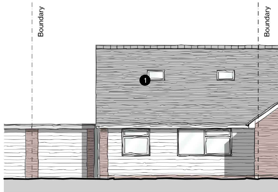
Front SW Elevation 1:100
